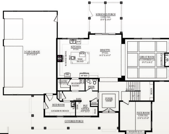
First Floor - 1,794 Sq. Ft.
